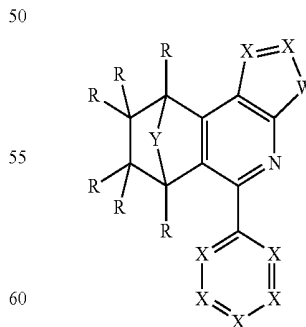
Formula (IIa2)
