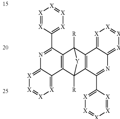
Formula (IIa1)
